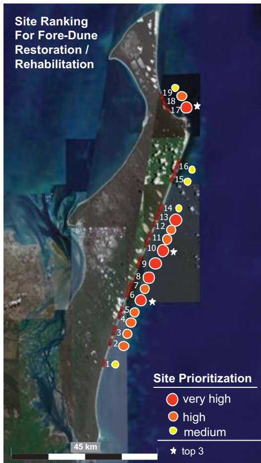
Fig. 5 Prioritization of camping zone for dune restoration and rehabilitation based on the extent of physical habitat damage (proportion of dune front destroyed), human pressure intensity (vehicle track density) and biological attributes (vegetation cover, plant species richness, ghost crab abundance). Graphical categorisation (medium, high, very high) is based on the 33 and 66 percentiles of total scores summed over the five variables above (cf. Table 1).
