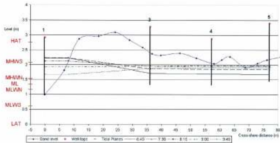
Figure 6: Main transect – wells 1 through 5. Water table levels are displayed for 2/12/06
