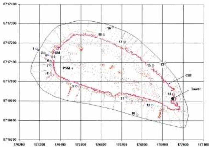
Figure 3: Raine Island map (WGS84 coordinates in metres) with location of groundwater monitoring wells (circles), survey data points (dots) and the Permanent Survey Mark 79041 (cross).
