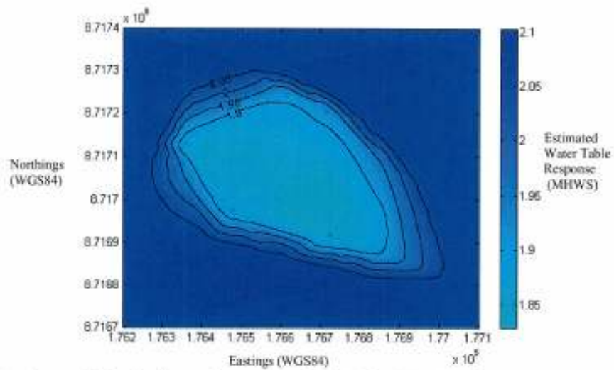
Figure 9: Estimated peak water table response (m above LAT) for a MHWS tide of 2.07m. Well locations are marked as crosses.
