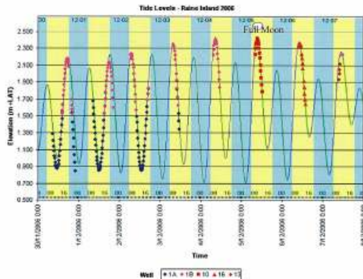
Figure 4: Tide measurements from the offshore wells 1,10,13 and 16 (dots) with the predicted astronomical tide level from WXTide32 (line).
