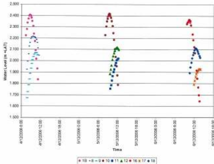
Figure 8: Measured water table response to high tide signal (offshore wells 1, 10 and 16) at wells 8, 9, 11, 12, 17 and 18
