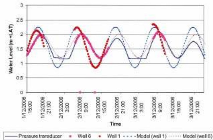
Figure 7: Pressure transducer recordings of water levels at well 6, compared to manual readings at wells 1 and 6 and simple model results for wells 1 and 6
