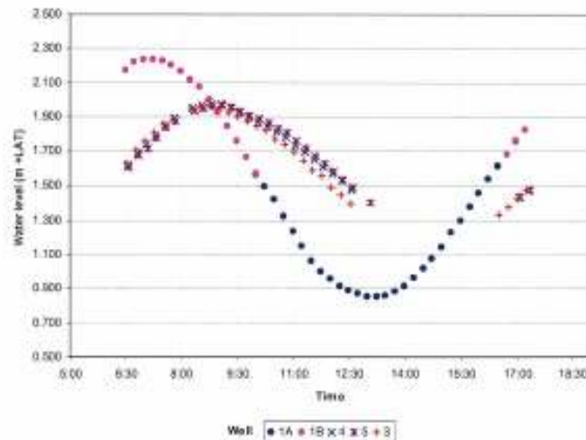
Figure 5: Water levels recorded along cross-shore transect (wells 1-5) on 2/12/06
